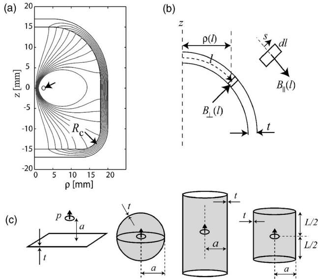
FIG. 1. (a) Magnetic field lines inside a high-permeability ( \mu_r=1000 ) shield with cylindrical symmetry. Mirror symmetry with respect to a transverse plane is not assumed. The field is generated by a current loop of radius 2.5 mm centered on the z axis, carrying 1 A dc; the small circle indicated by the arrow shows the cross section of the wire. The field lines closest to the wire are not shown. The 11 field lines that are shown enclose magnetic flux of n\Delta\Phi , n=1, 2, \dots, 11 , where \Delta\Phi=10^{-10} Wb. (b) Cross section of the shield in the \rho - z plane. (c) Four geometries considered in the power loss calculation: infinite plate, sphere, infinite cylinder, and finite closed cylinder. The cylinders and the sphere are hollow shells of thickness t .
