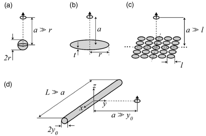
FIG. 2. Definition of geometries used to calculate magnetic field noise from (a) a small solid sphere, (b) a thin disk with arbitrary diameter, (c) a square array of small thin disks covering an infinite plane, and (d) a long, thin wire with a circular cross section. In (c), the small disks have thickness t , are close-packed, but are electrically isolated from each other.
