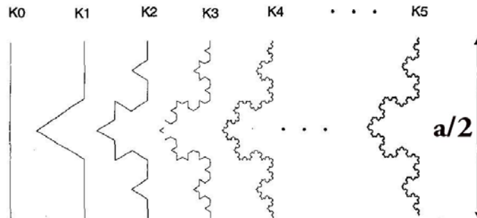
Figure 3: The pattern of one arm of a Koch fractal dipole antenna. From [6].
