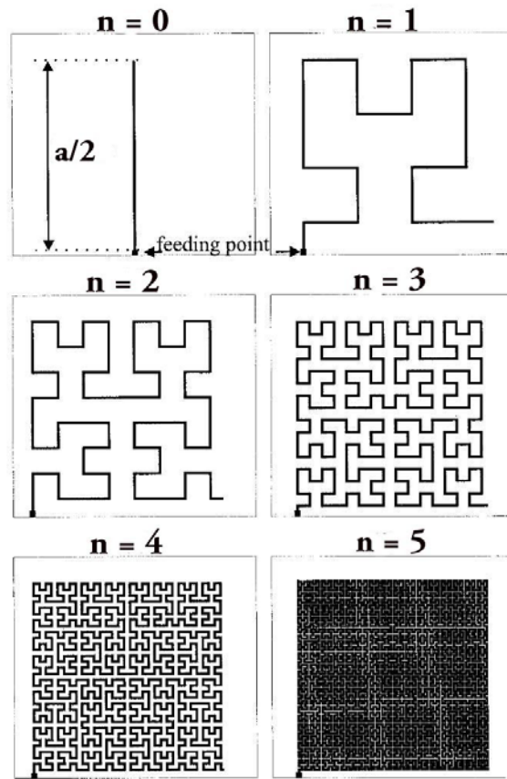
Figure 2: The pattern of one arm of a Hilbert fractal dipole antenna. From [5]. For the calculations in the text, the origin is taken at the feed point, the x axis is horizontal and the y axis is vertical. The patterns of fractal dipole antennas are obtained by reflecting the patterns in the figure about the x axis.
