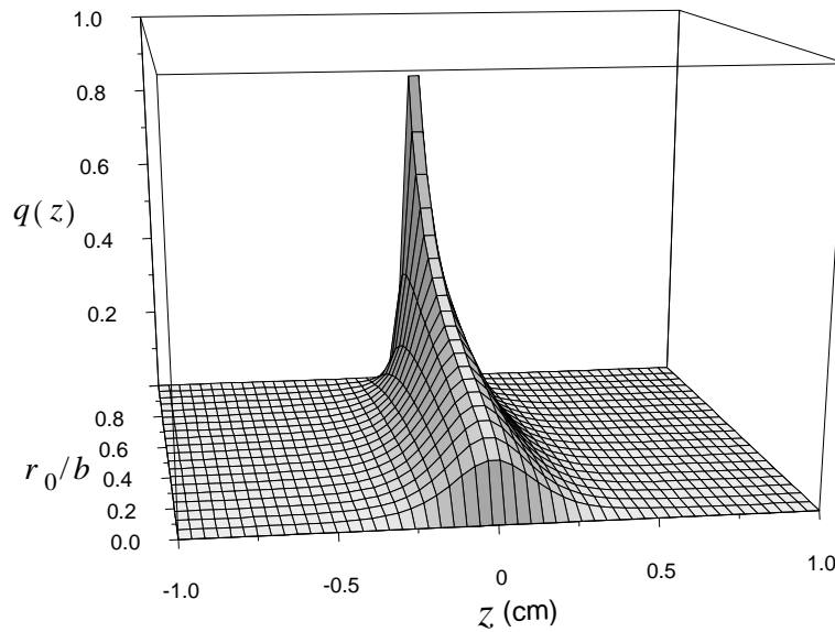
Figure 1: The induced charge distribution (26) on the cathode of a straw tube chamber of radius b = 0.25 cm due to positive ion charge at radius r_0 .
